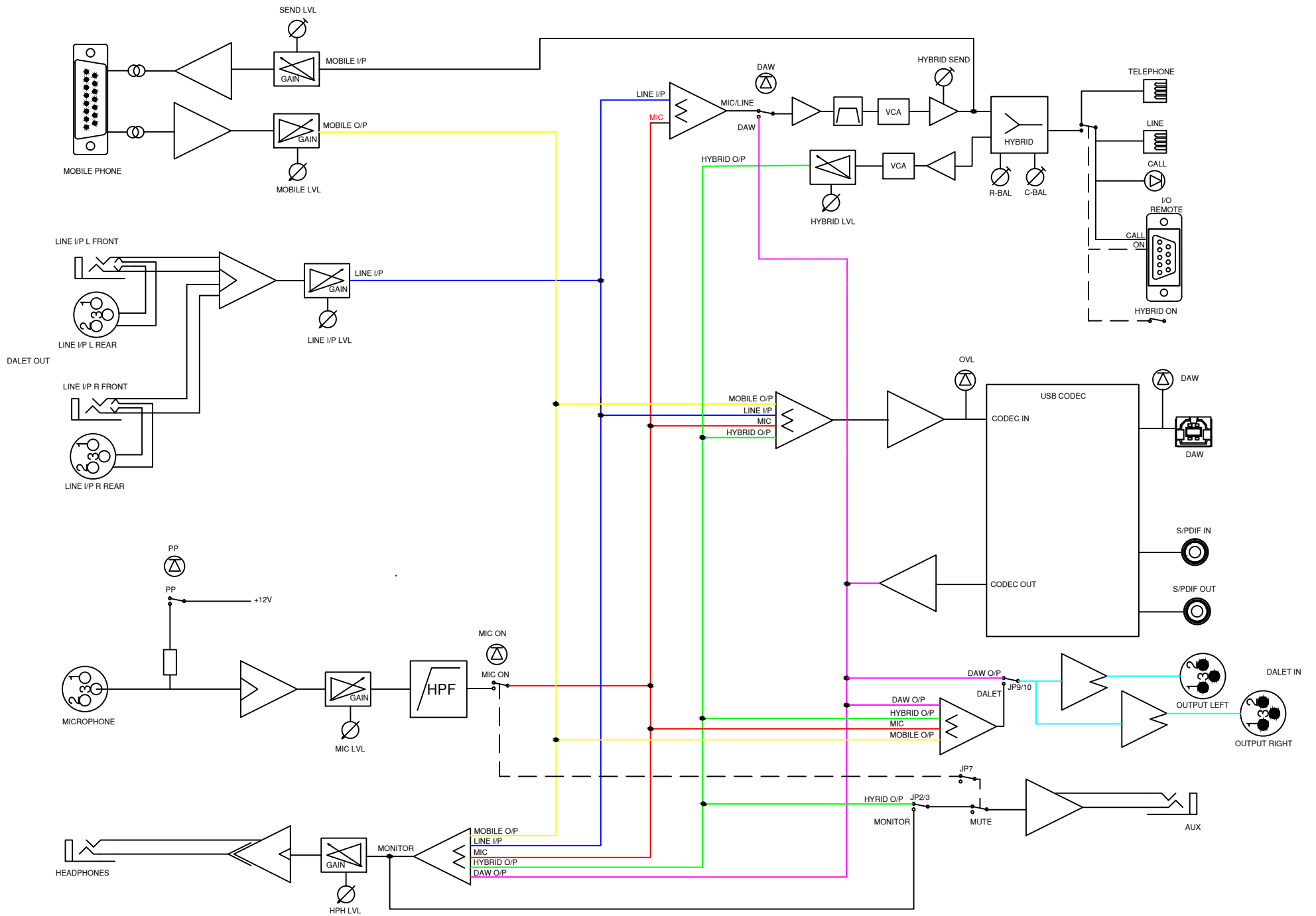
BLOCK DIAGRAM EA916 JOURNALIST UNIT
